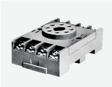
DIN Rail 8-PIN Socket (Time-S3-08)
